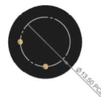
Product Dimensions All dimensions in mm All tolerances ±0.15 mm
